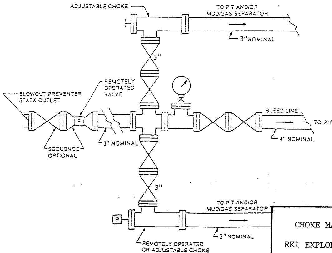
FIGURE K4-2. Typical choke manifold assembly for 5000 rated working pressure service — surface installation.
