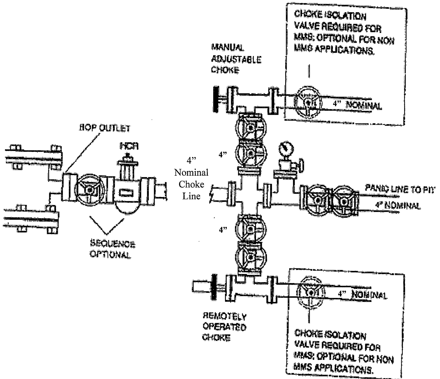
Exhibit E-1 – Choke Manifold Diagram Cave Lake 13 Federal Com No. 2 Cimarex Energy Co. of Colorado 13-16S-28E SHL 1980' FSL & 330' FEL BHL 1980' FSL & 330' FWL Eddy County, NM
