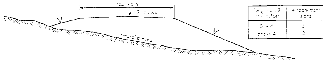
Embankment Section
