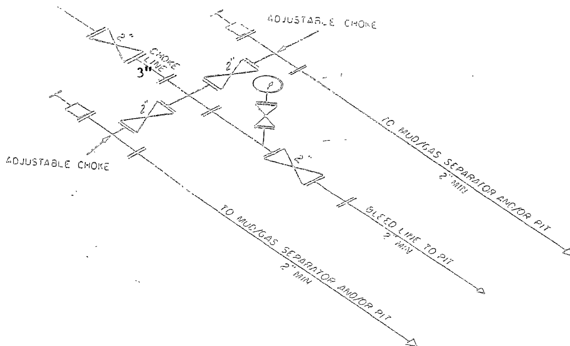
2M CHOKE MANIFOLD EQUIPMENT — CONFIGURATION OF CHOSES
