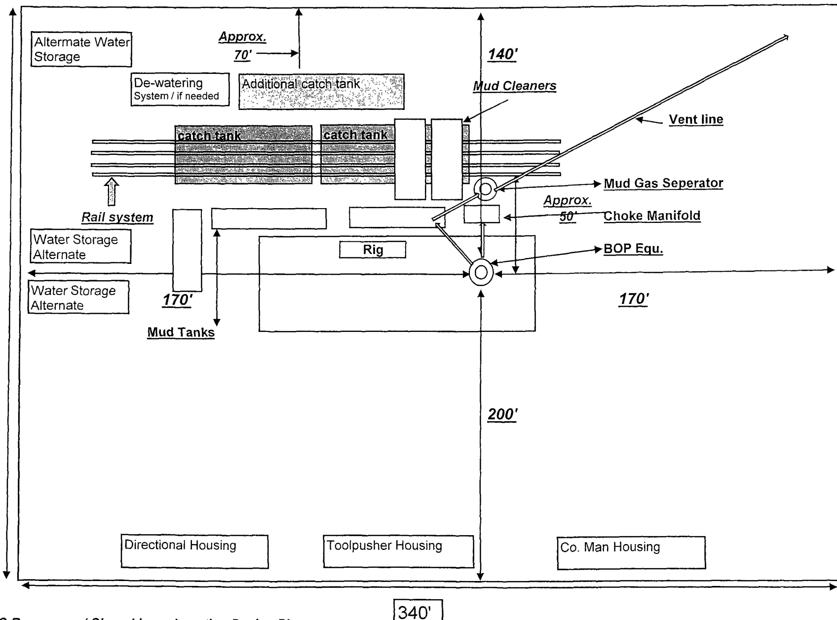
EOG Resources / Closed Loop Location Design Plan
