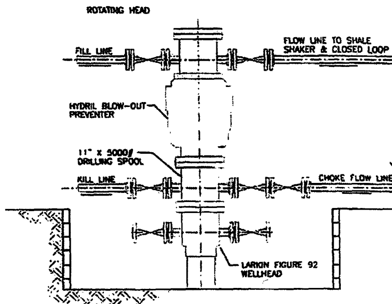
WELLHEAD ELEVATION
