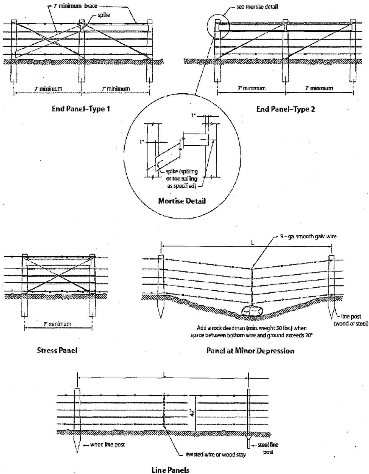
Figure 1. Recommended construction standards for enclosure fences in livestock areas.
