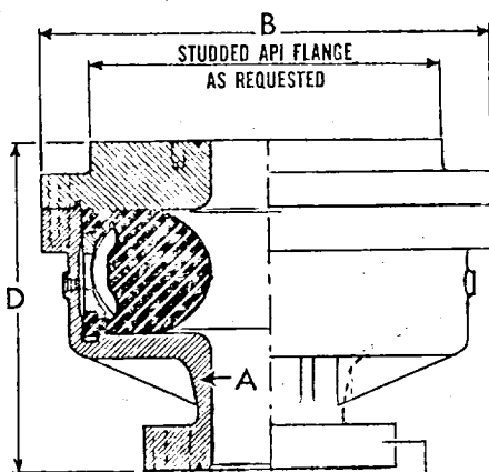
SERIES 900 API NOM "C" FLANGE SLOTTED FOR SERIES 400 OR 600 BOLTING
