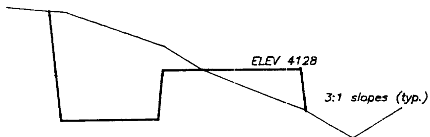
W-E CROSS-SECTION, VERTICAL EXAGGERATION FACTOR 10
