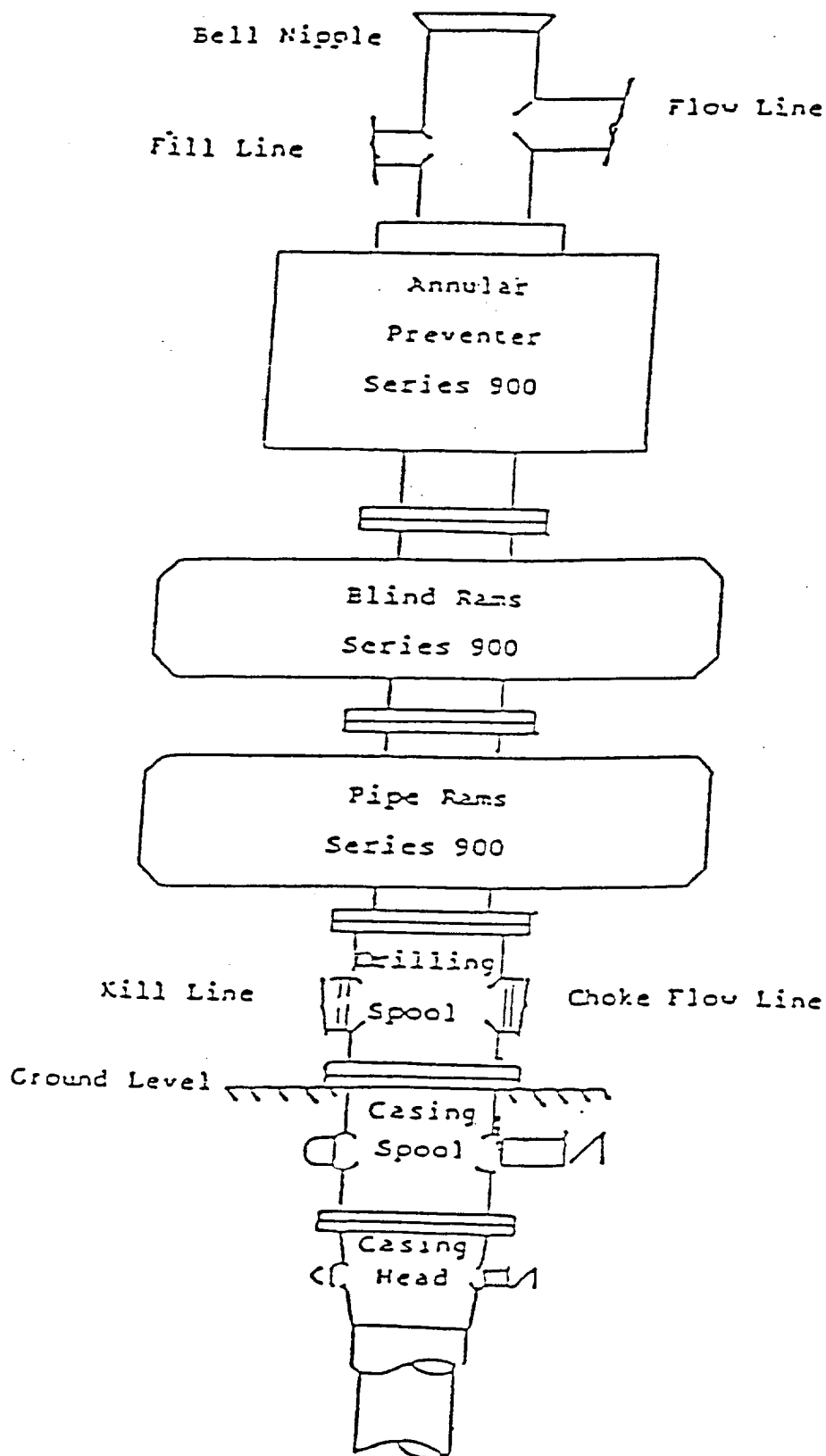
BLOWOUT PREVENTER STACK
