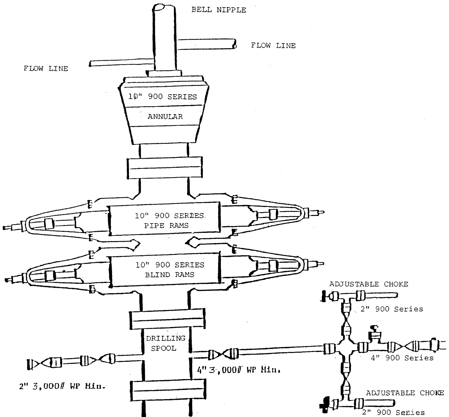
BOP & Choke Manifold Schematic Mewbourne Oil Company Empire "18" State #7 Section 18/17S/31E Eddy County, New Mexico
