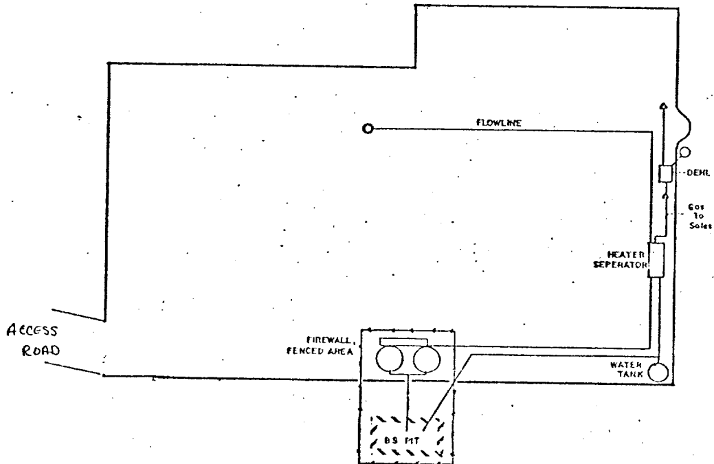
TANK BATTERY LAYOUT
