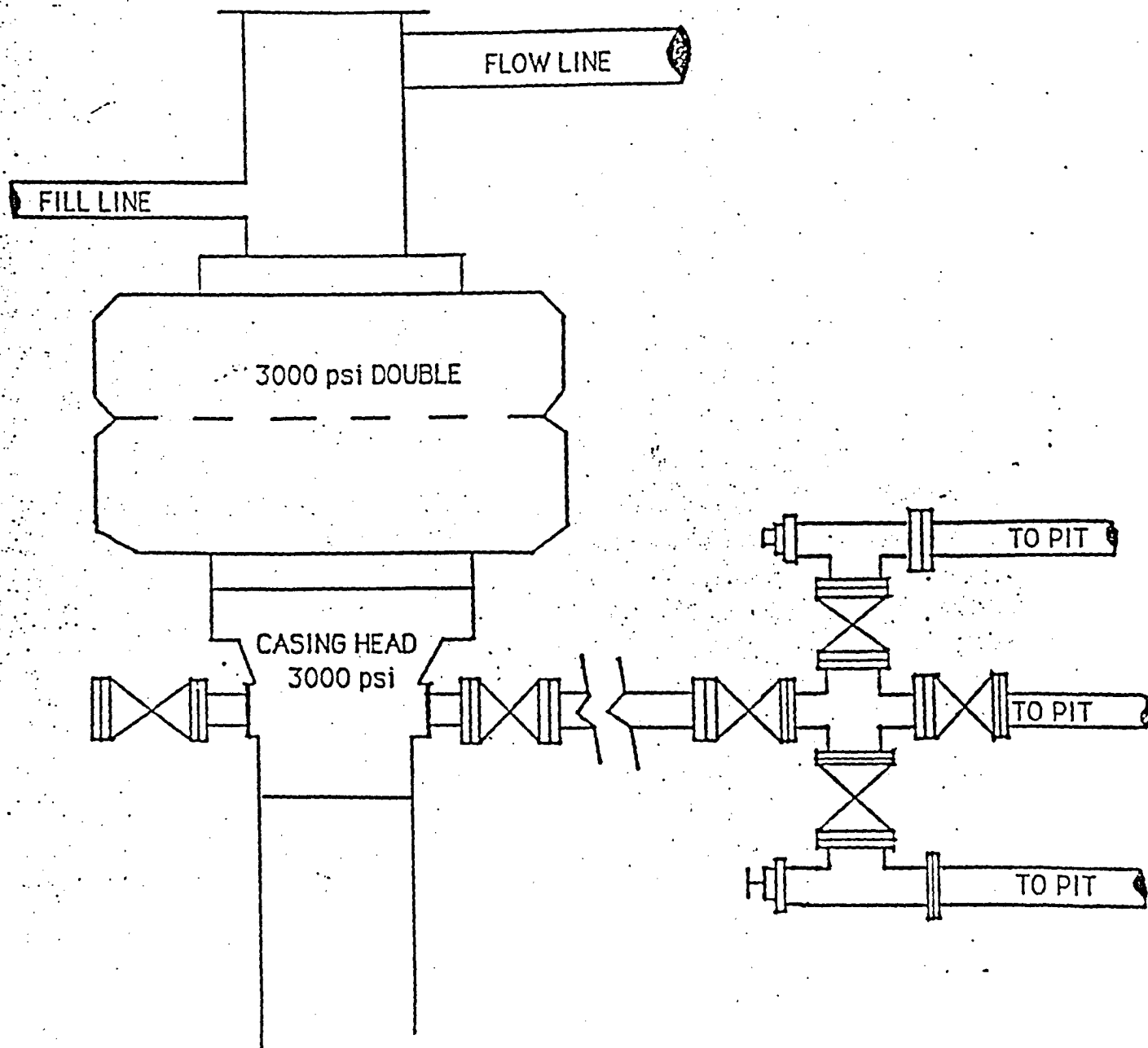
BLOWOUT PREVENTER
