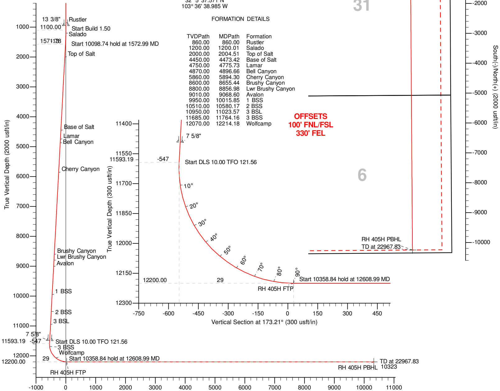
Vertical Section at 173.21° (2000 usft/in)
