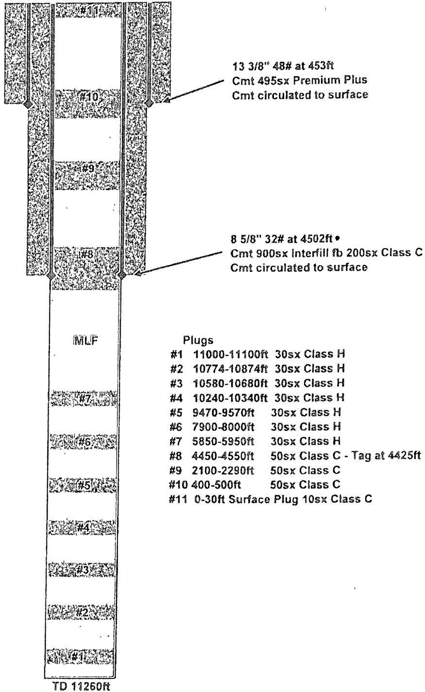
Current Well Diagram
