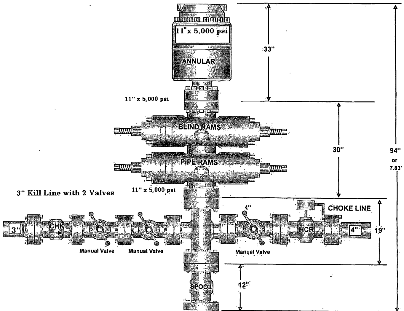
Exhibit 2.2 11" x 5M BOPE stacking configuration
