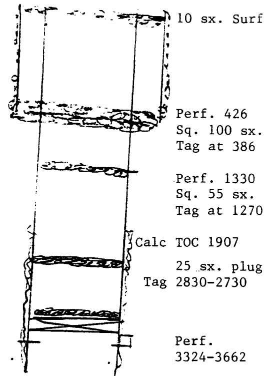
AFTER PLUGGING
