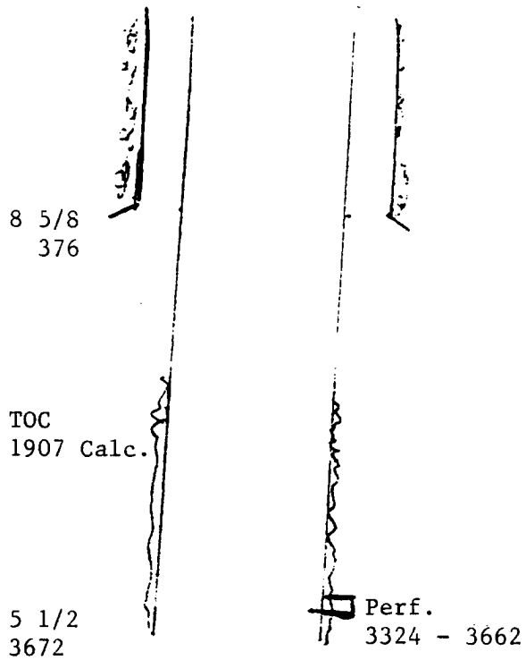
BEFORE PLUGGING
