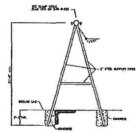
TANK VENT PIPE SUPPORT NOT TO SCALE
