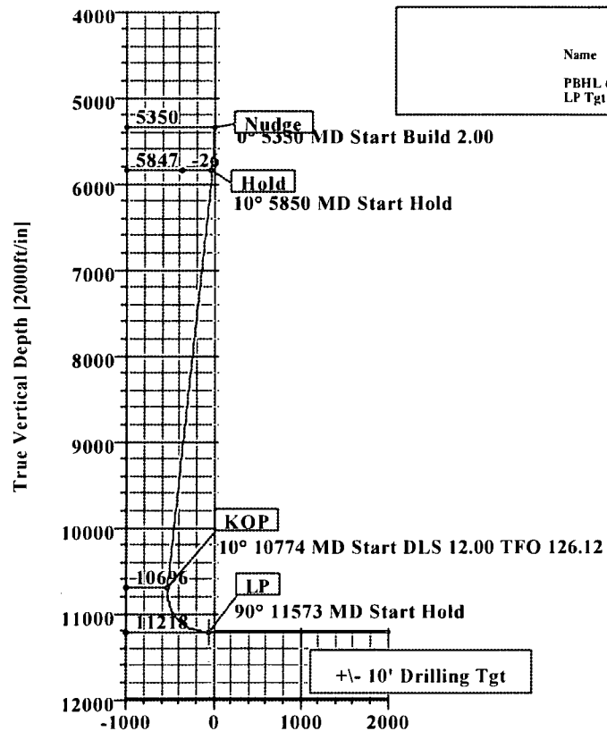
Vertical Section at 356.35° [2000ft/in]
