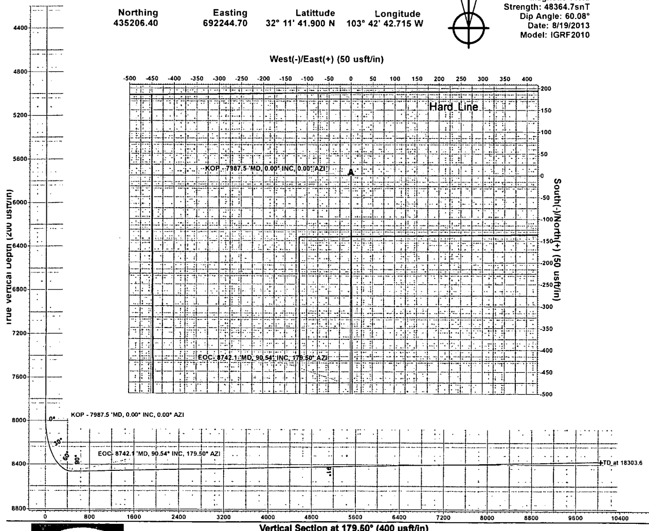
Vertical Section at 179.50° (400 usft/in)
