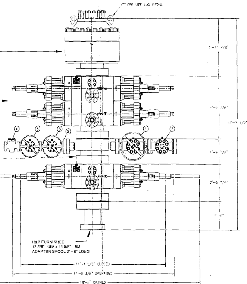
13 5/8 - 10M BOP STACK WITH 13 5/8 - 5M ANNULAR
