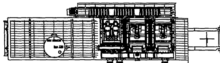
Mud Tank/Generator
