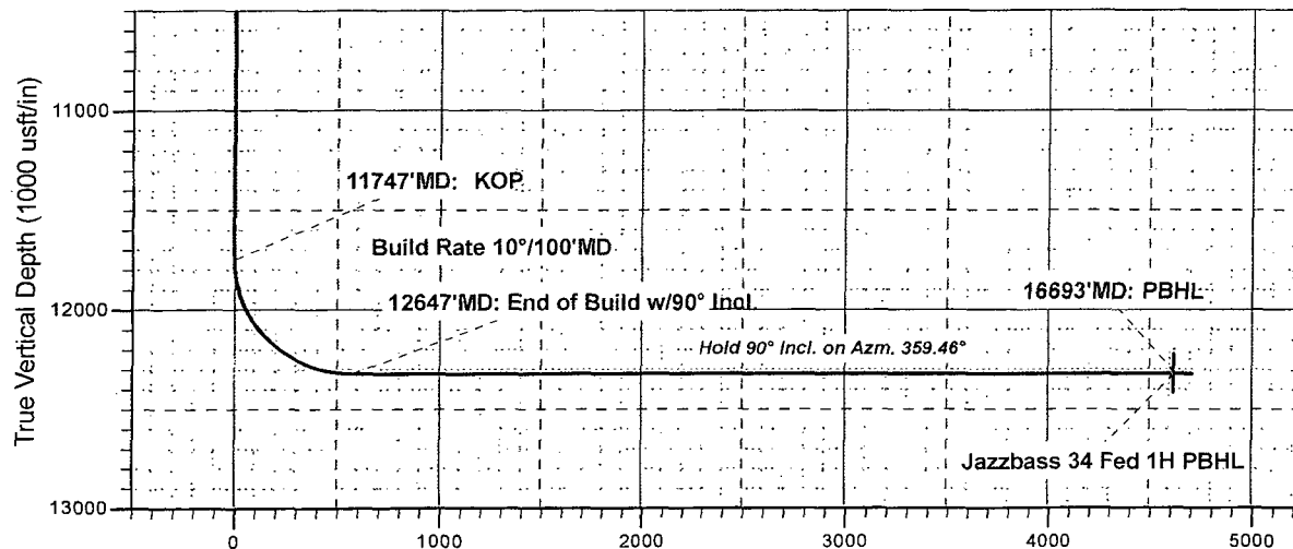
Vertical Section at 359.46° (1000 usft/in)
