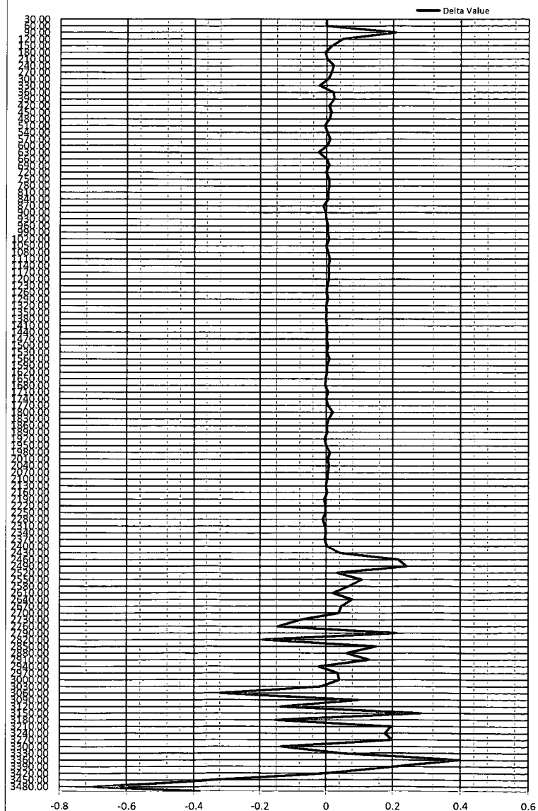
Cabra Loca 11 B3PA St Com #1H Delta T Log
