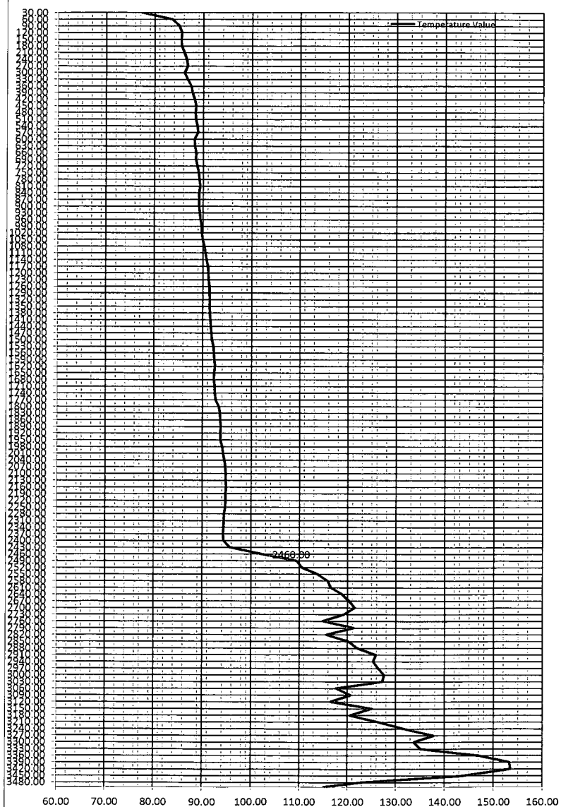
Cabra Loca 11 B3PA St Com #1H Temp Log
