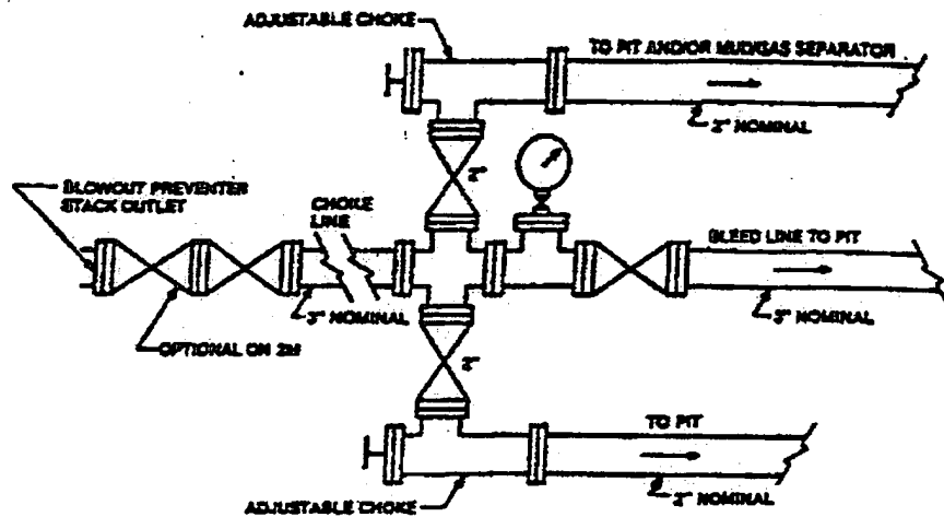
Typical choke manifold assembly for EM WP system
