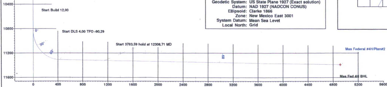
Vertical Section at 184.86° (200 ft/in)
