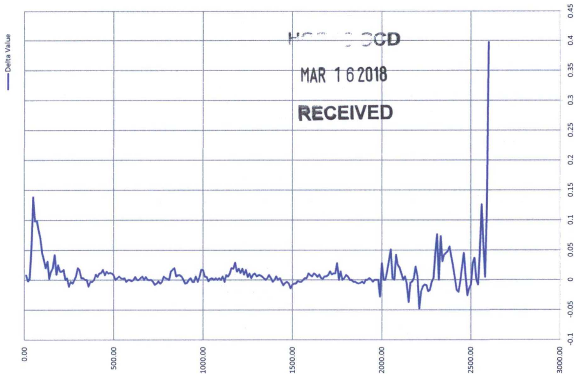
"Wildhog BWX State Com 002H" Delta T Log
