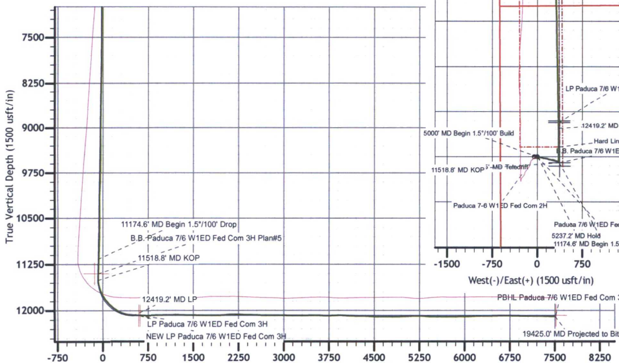
Vertical Section at 2.51° (1500 usft/in)
