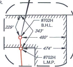
DETAIL VIEW B SCALE: 1" = 500'
