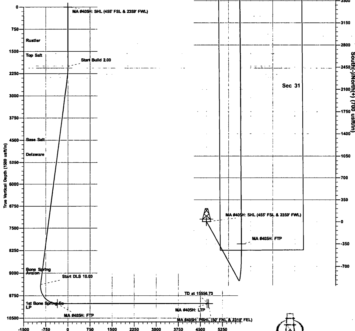
Vertical Section at 359.61° (1500 usft/in)
