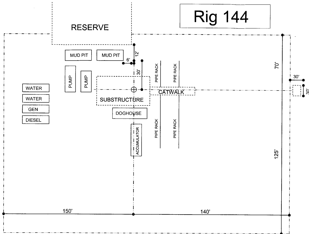
Exhibit D – Rig Layout Pipeline B5 Federal No. 1 Cimarex Energy Co. of Colorado B-5-19S-34E 660' FNL & 1650' FEL Lea County, NM
