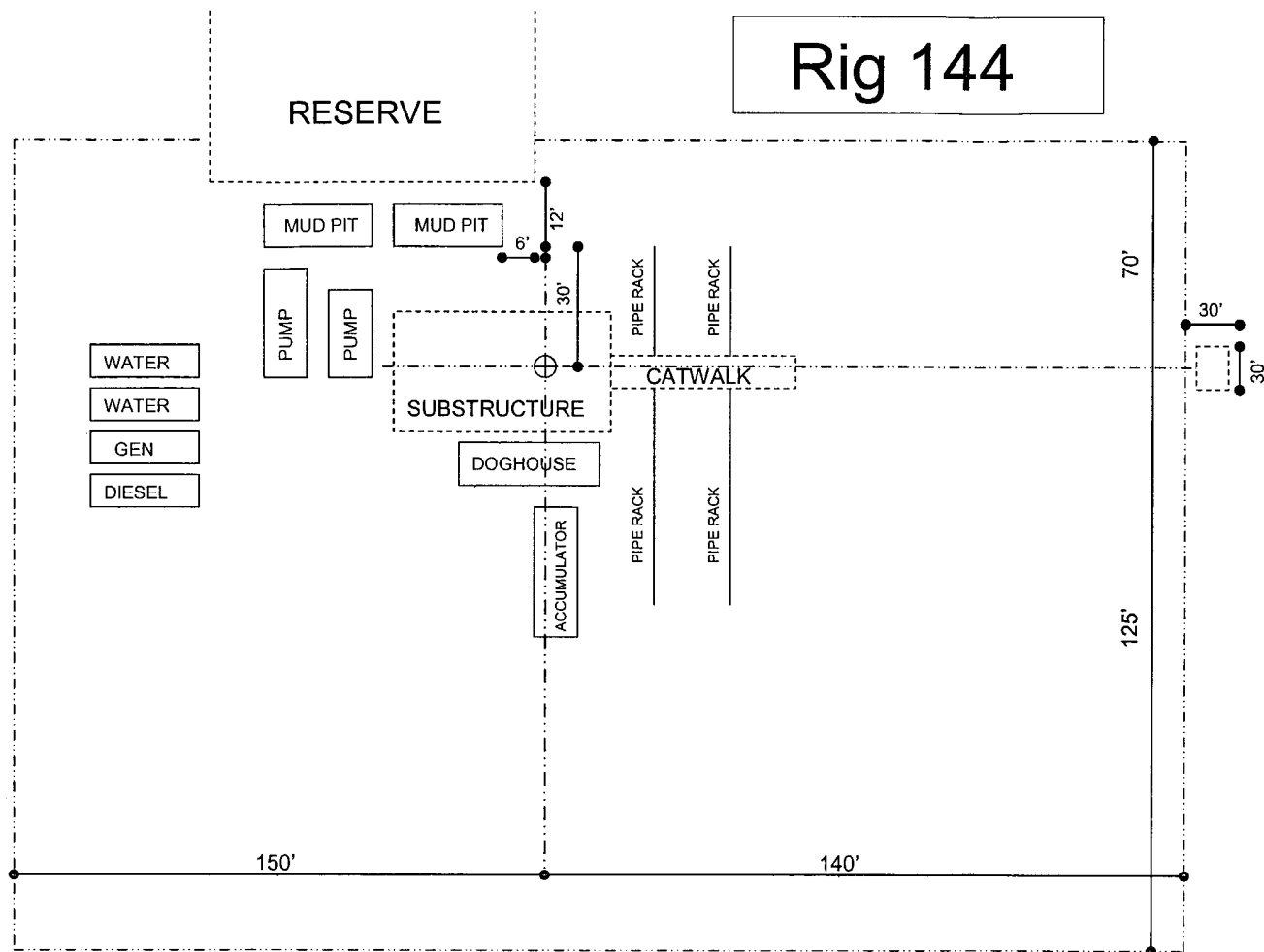
Exhibit D – Rig Layout Pipeline B5 Federal No. 2 Cimarex Energy Co. of Colorado K-5-19S-34E 1650' FSL & 1980' FWL Lea County, NM
