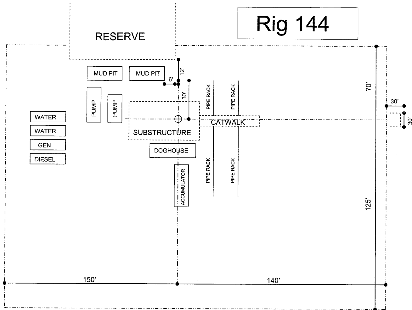
Exhibit D – Rig Layout Pipeline B6 Federal No. 2 Cimarex Energy Co. of Colorado F-6-19S-34E 2310' FNL & 1980' FWL Lea County, NM
