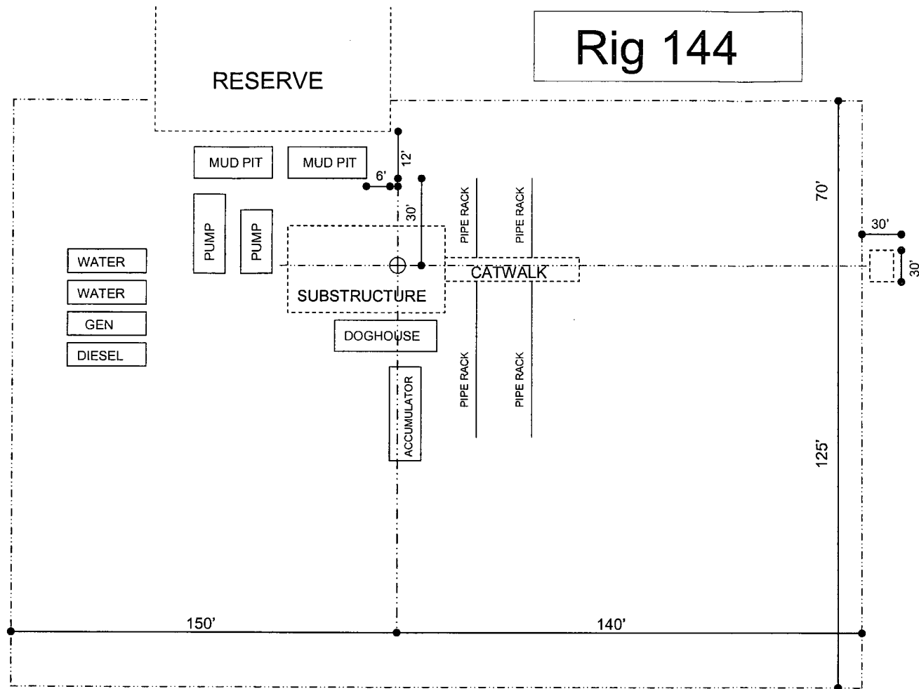
Exhibit D – Rig Layout Pipeline B6 Federal No. 2 Cimarex Energy Co. of Colorado G-6-19S-34E 1980' FNL & 1980' FEL Lea County, NM
