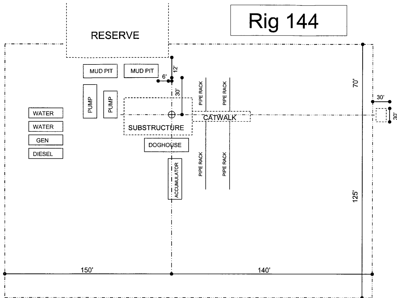
Exhibit D – Rig Layout Pipeline B18 Federal No. 7 Cimarex Energy Co. of Colorado E-18-19S-34E 1980' FNL & 510' FWL Lea County, NM
