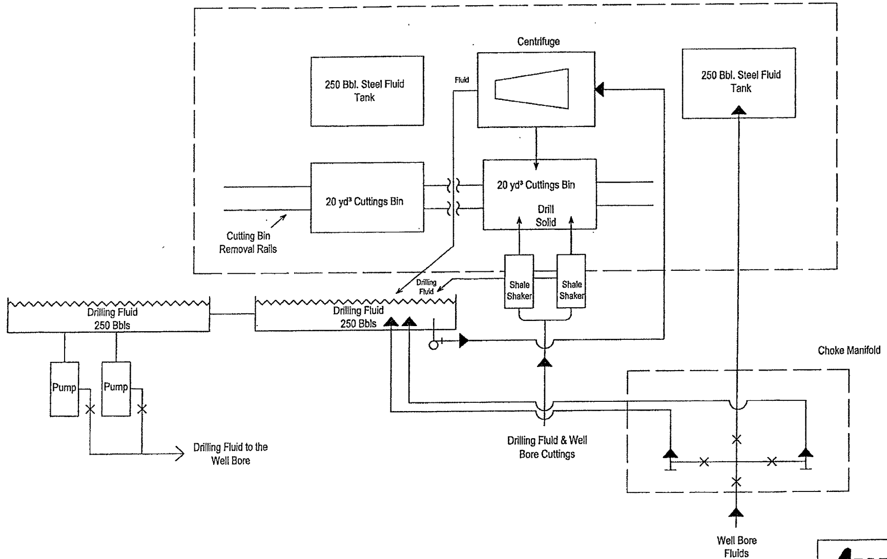
Figure 1 New Mexico Typical Closed-Loop System
