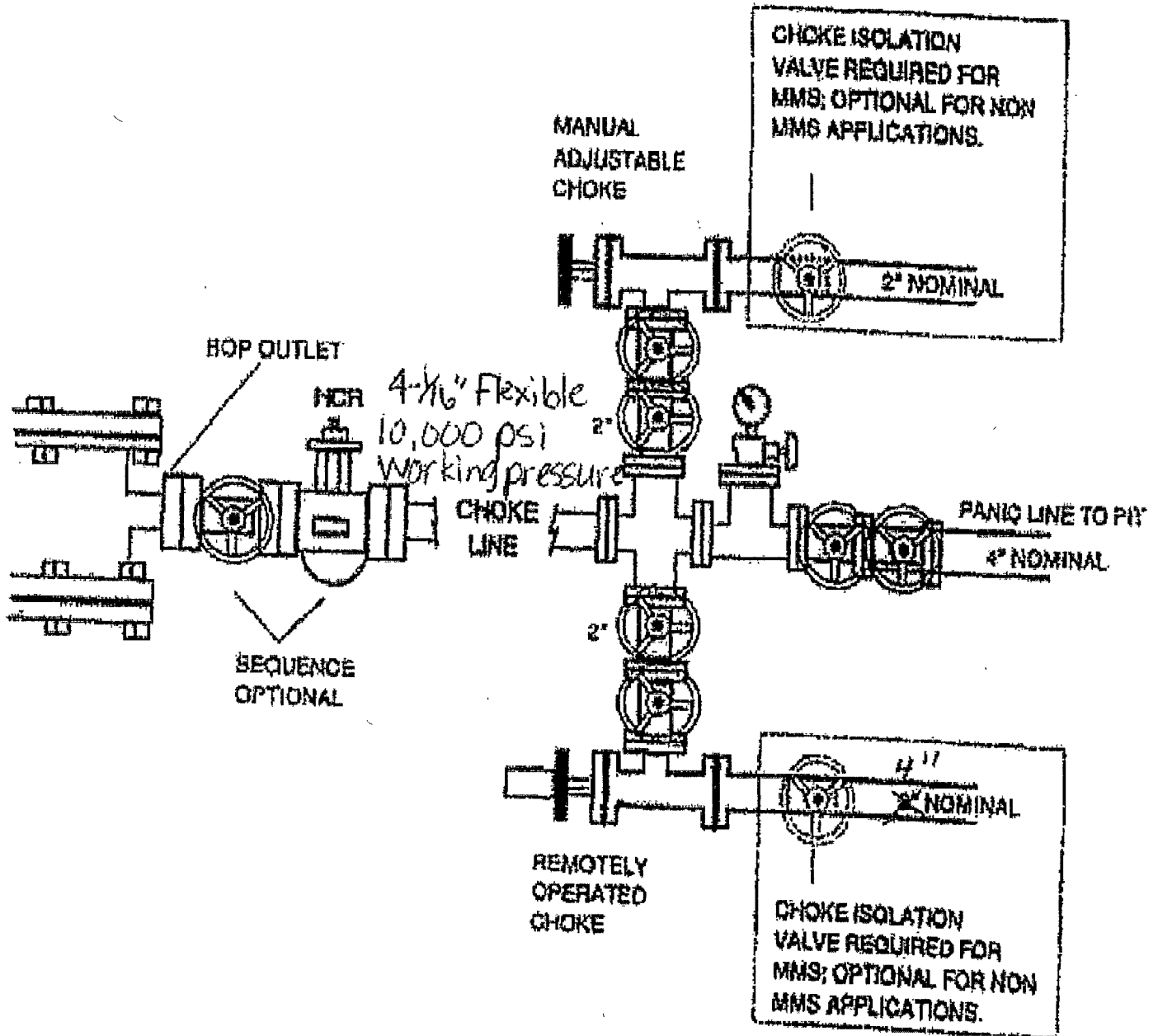
Exhibit E-2 – Choke Manifold Diagram San Jacinto 4 Federal Com No. 1 Cimarex Energy Co. of Colorado 4-15S-31E SHL 375 FNL & 330 FWL BHL 375 FNL & 330 FEL Chaves County, NM
