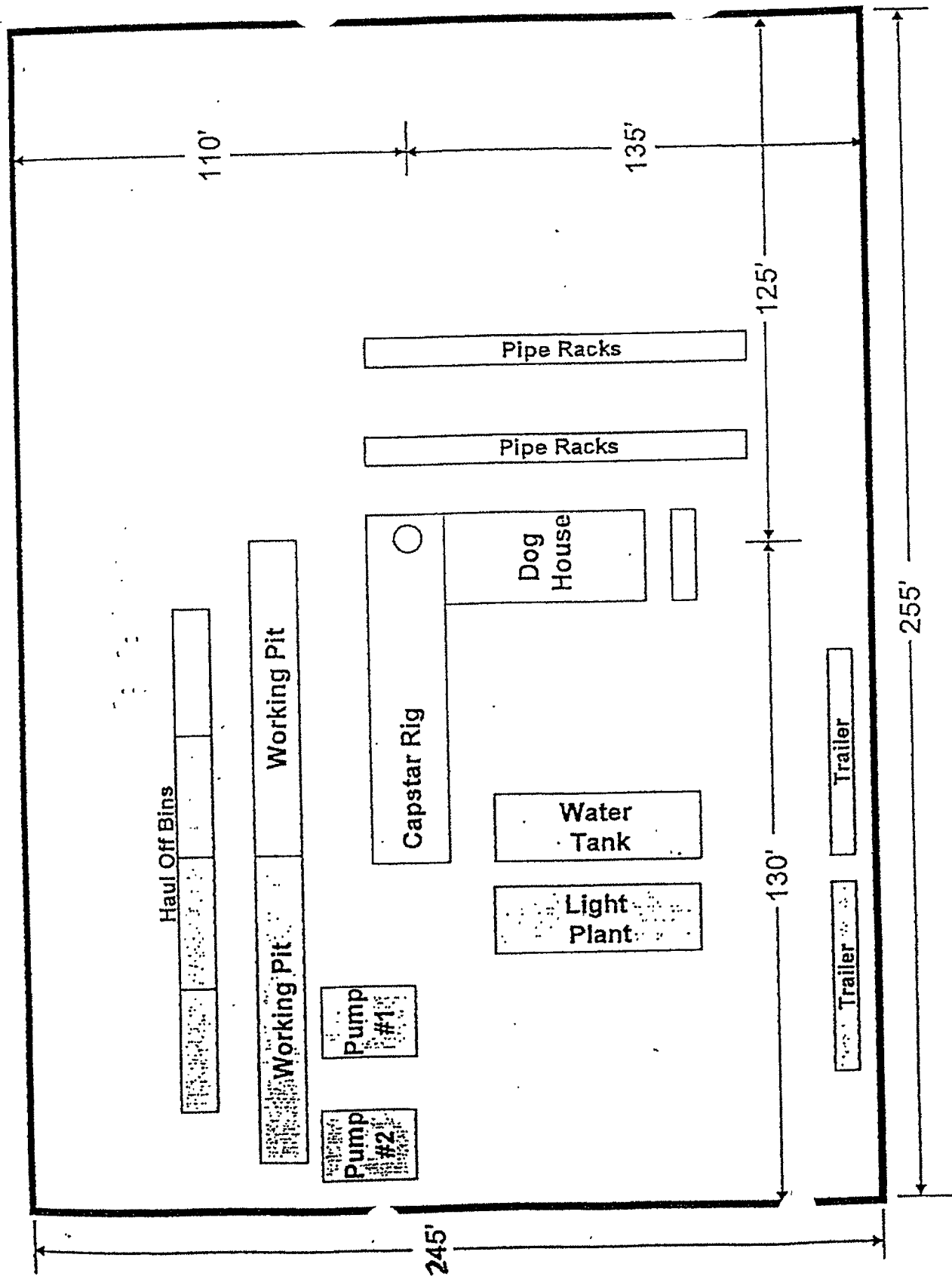
Rig Layout Diagram
