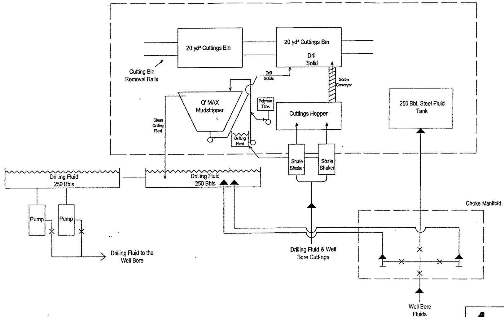
Figure 1 New Mexico Q' MAX Closed-Loop System
