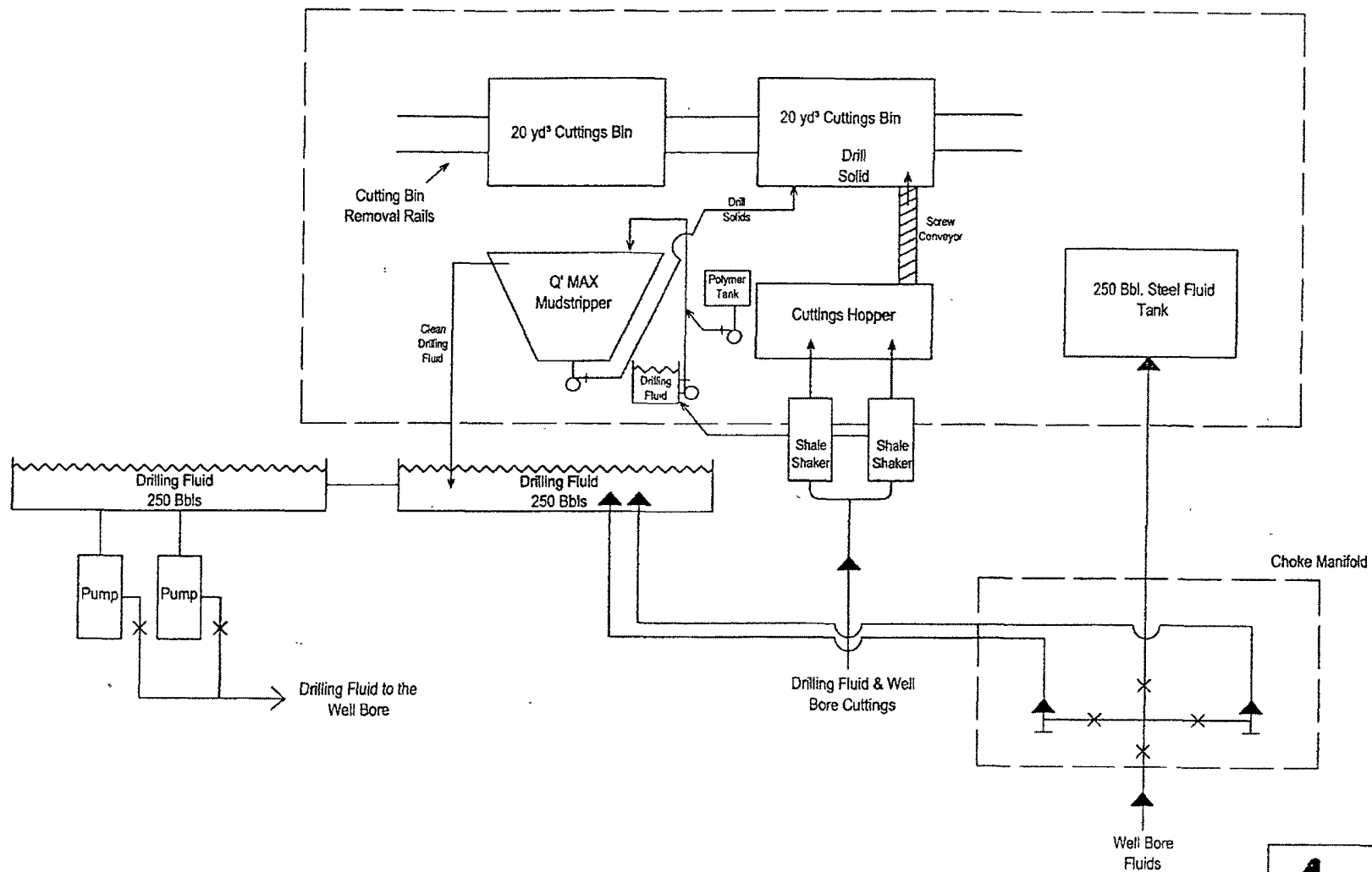
Figure 1 New Mexico Q' MAX Closed-Loop System
