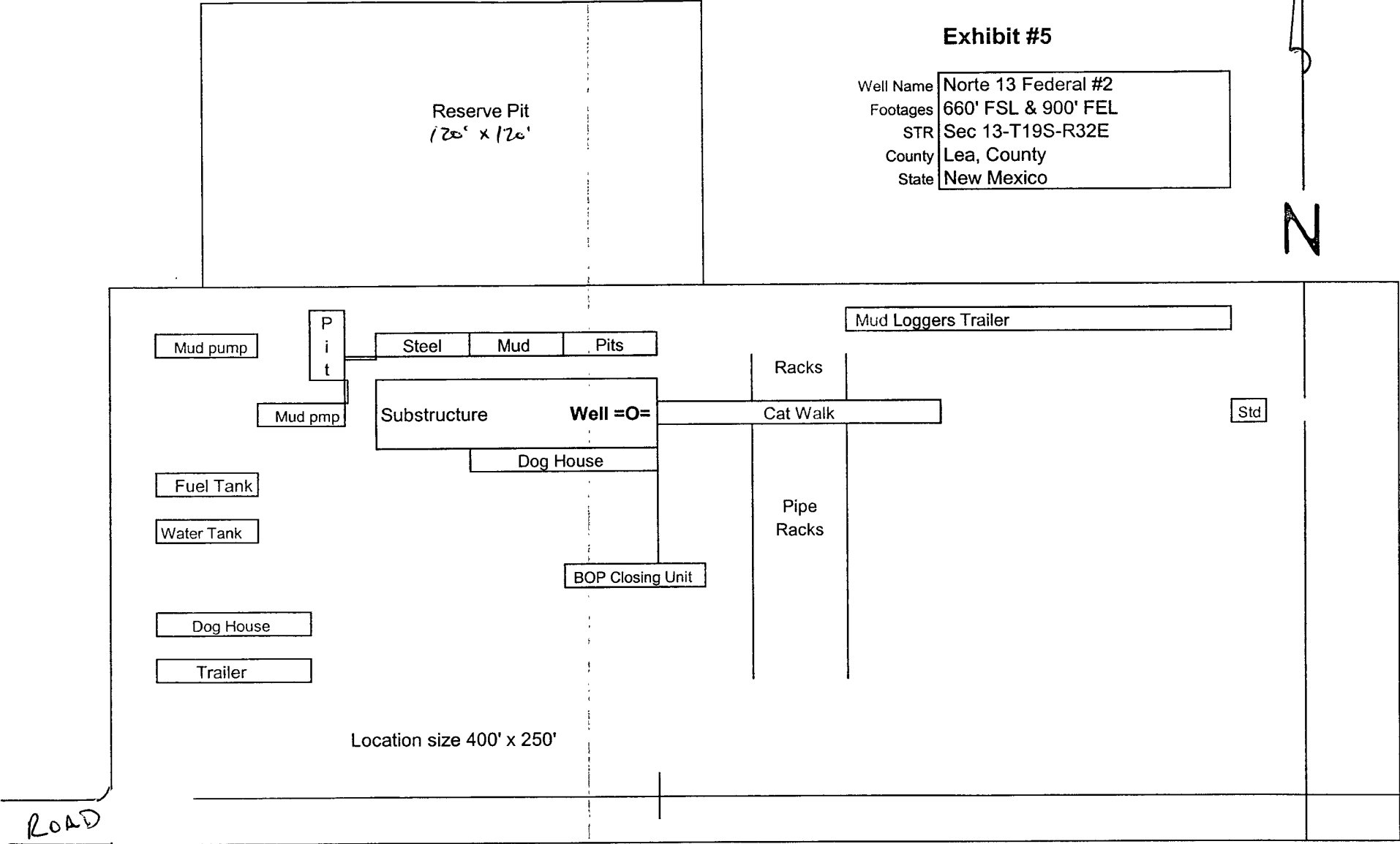
Rig Location Schematic
