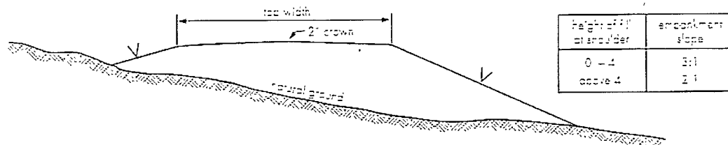
Embankment Section
