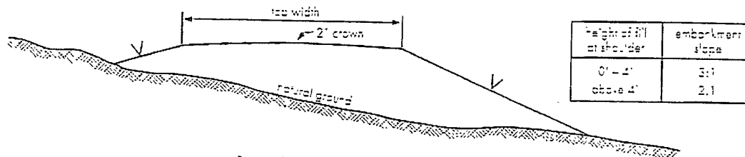
Embankment Section
