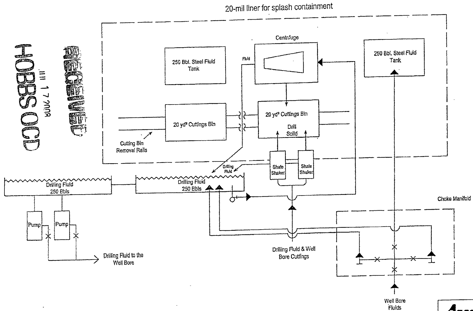
Apache CORPORATION Figure 1 New Mexico Typical Closed-Loop System
