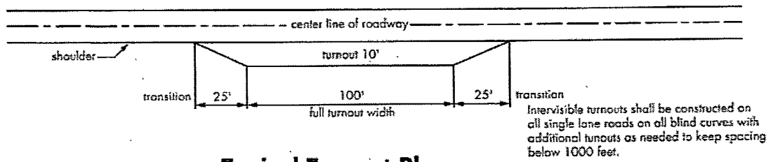
Typical Turnout Plan
