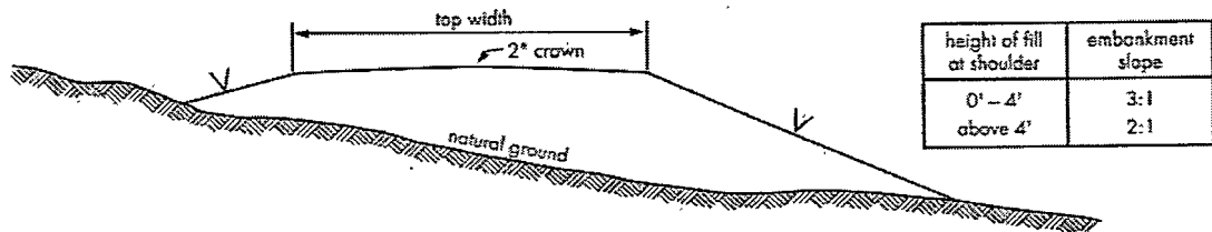
Embankment Section
