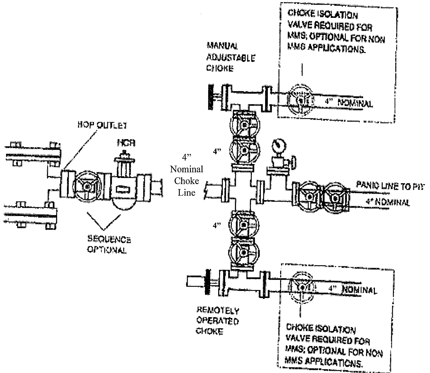
Exhibit E-1 – Choke Manifold Diagram Independence 8 Federal Com No. 1 Cimarex Energy Co. of Colorado 8 & 9, 15S-31E SHL 510 FNL & 2310 FEL, 8-15S-31E BHL 660 FNL & 330 FEL, 9-15S-31E Chaves County, NM
