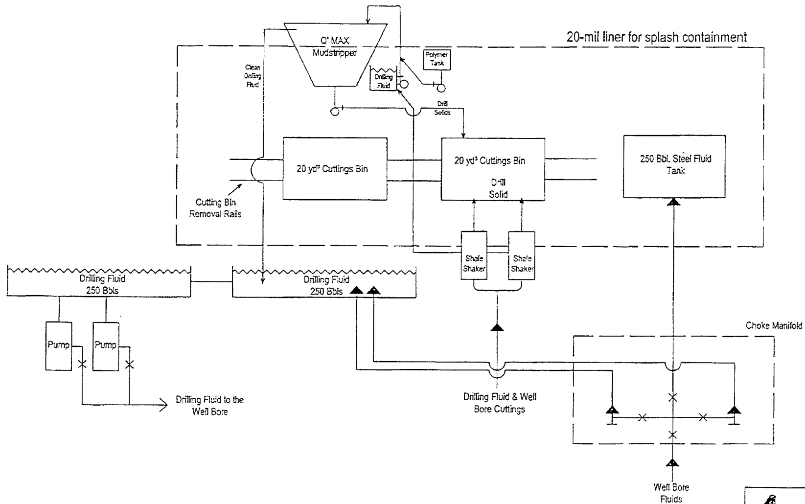
Figure 1 New Mexico Q' MAX Closed-Loop System
