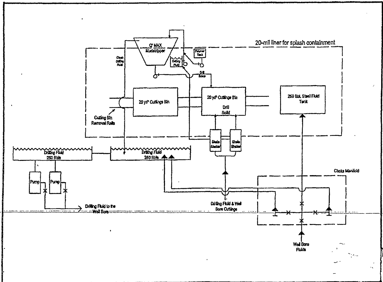
Pedernales Production, LP New Mexico Closed Loop System
