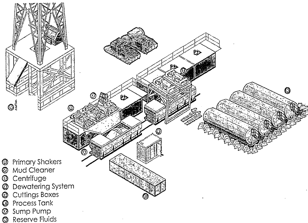
Closed Loop Schematic
