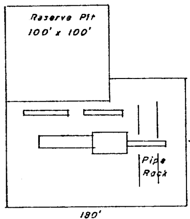
PAD DETAIL
